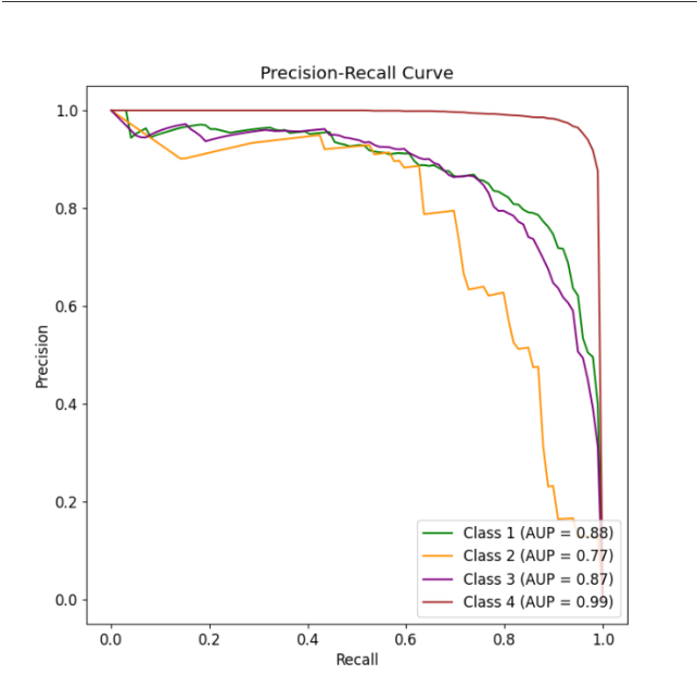
PR curve
